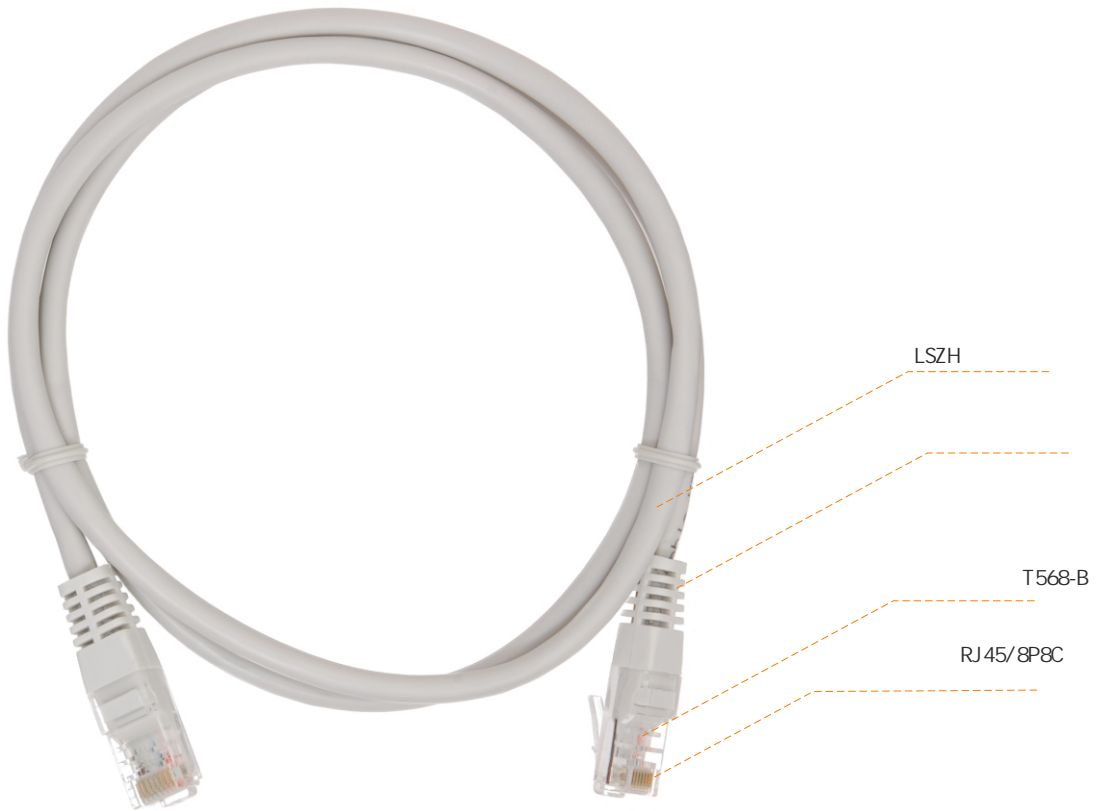
EC-PC4UD55B-BC-LSZH-XXX-GY-10
